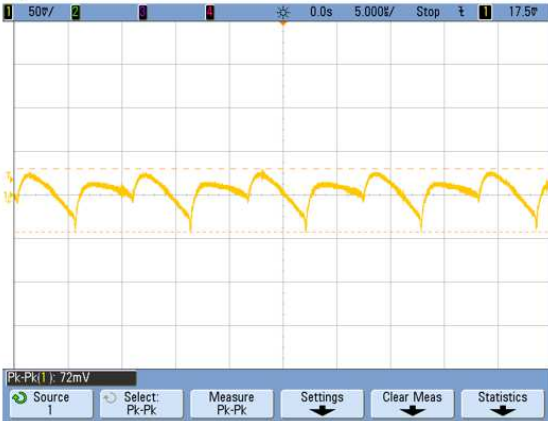
Switching frequency ripple rated load
