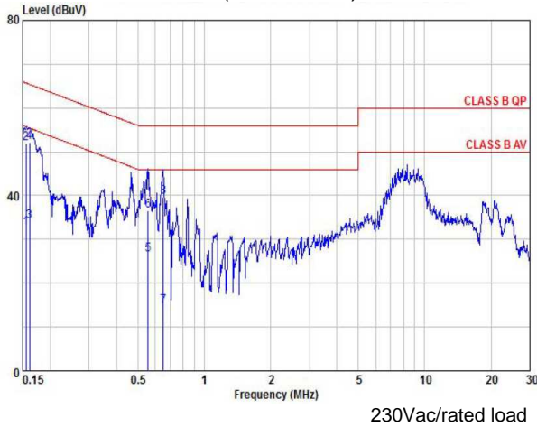
EMI: EN55011 "B" (Conduction)
