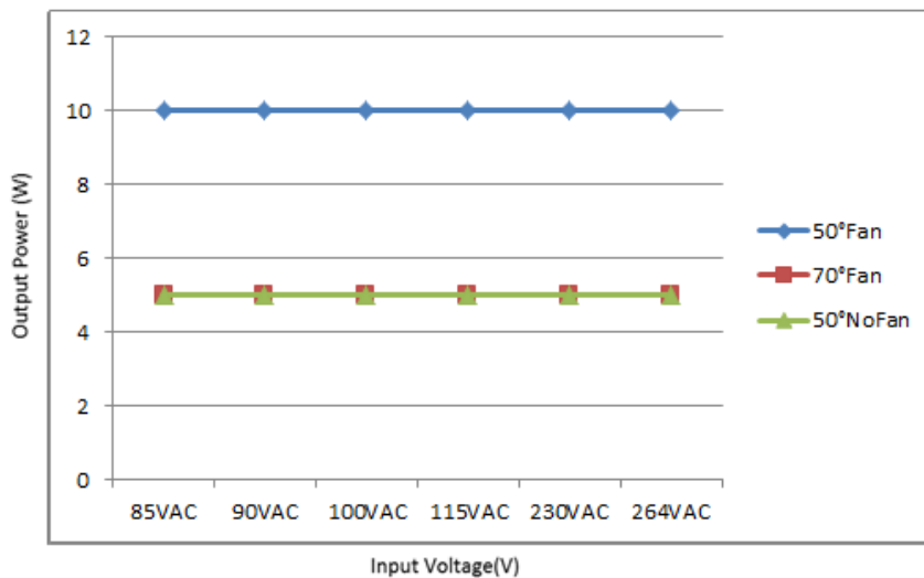
Performance curves of MPM-U655
