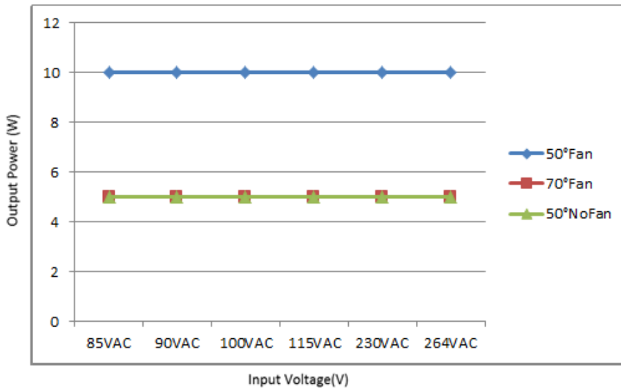
Performance curves of MPM-U656
