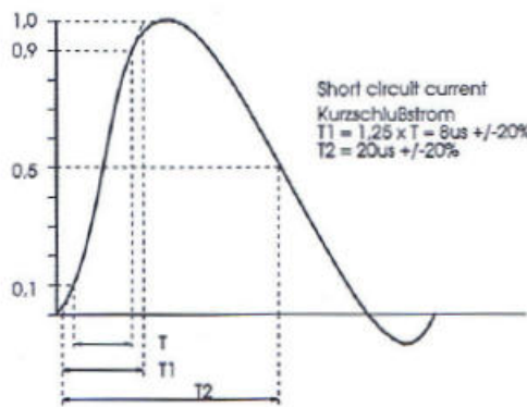
Waveshape definition current Kurvenform Stoßstrom
